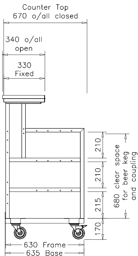
Intermediate "cut-away" supports for Front Counter
