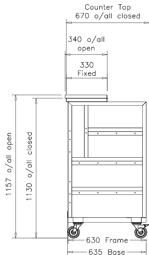
End supports for Front Counter units.
